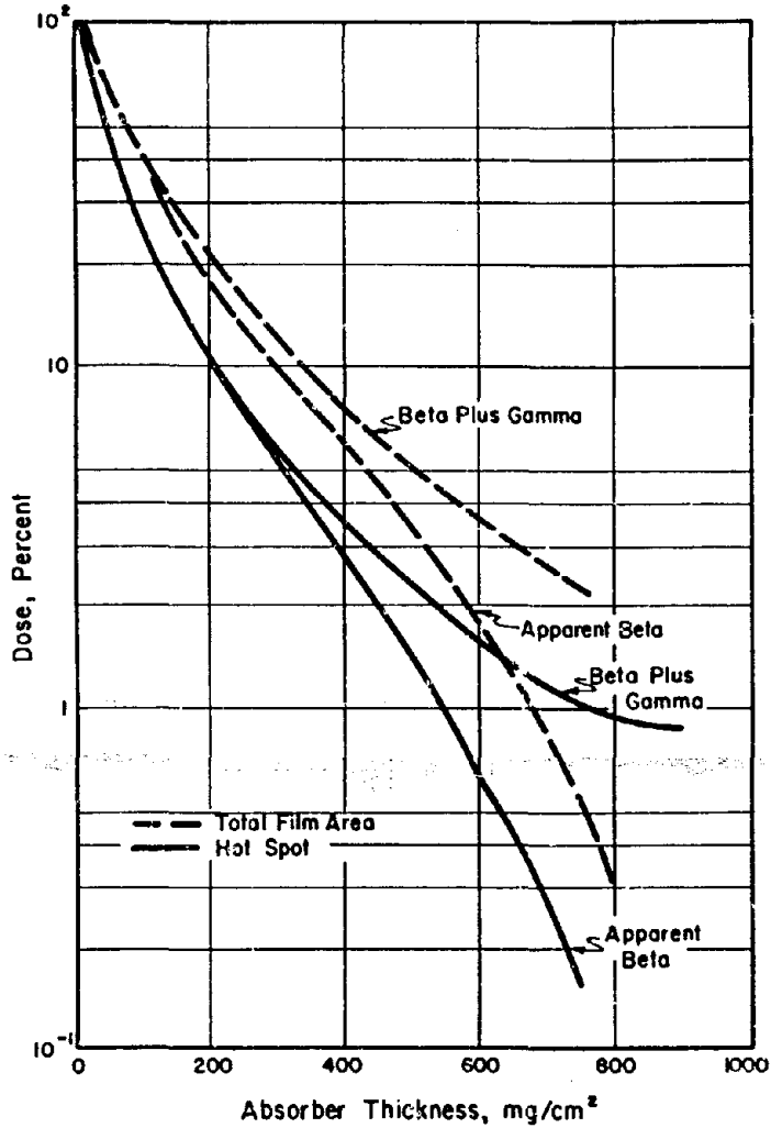
Figure 3.3 Depth-dose measurements on leading edge of B-57B.
